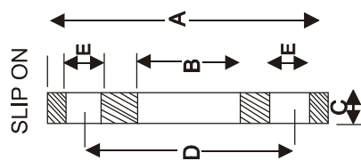
BS 10 Pipes
