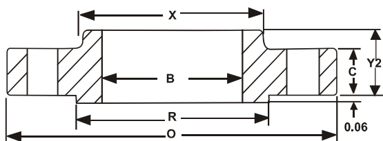
Slip On
