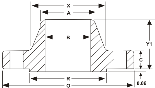
Weld Neck
