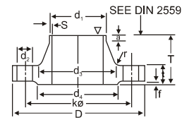
WELDING NECK
