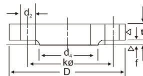
BLIND
