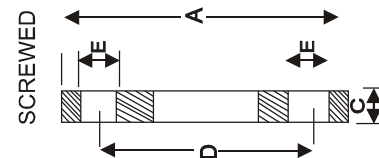
BS 10 Pipes
