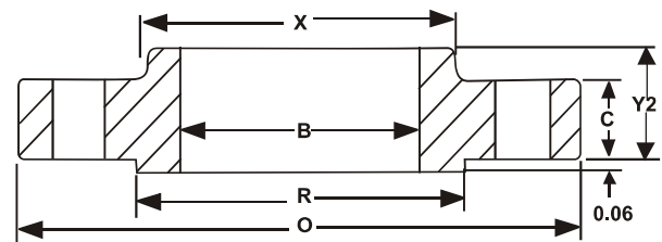
Slip On
