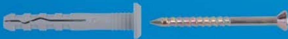
Nylon Hammer Fixing,Mushroom Head Model: HFS0640M-HFS0680S Sleeve: Nylon 6. Screw: Blue/Yellow Zinc Plated.
