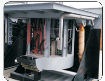
Furnace Housing
