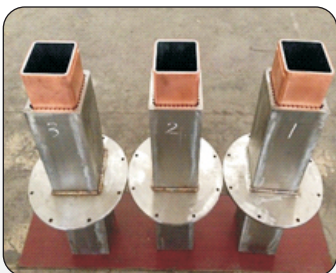
Mould Inner Casing
