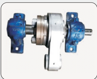
Oscillation Assembly
