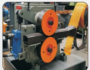
Pinch Roll
