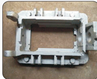
Adaptor + Housing
