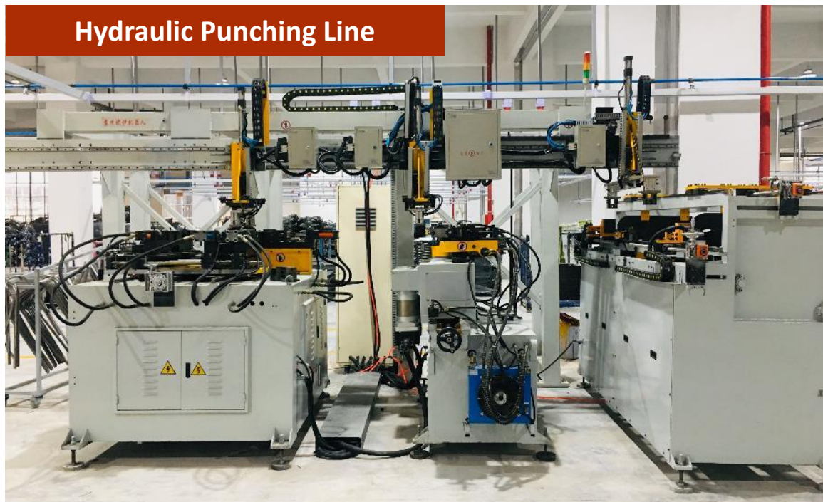
Tube Tapering Production Line
