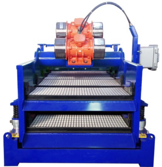
■ 双层振动筛 Double Deck Shaker
